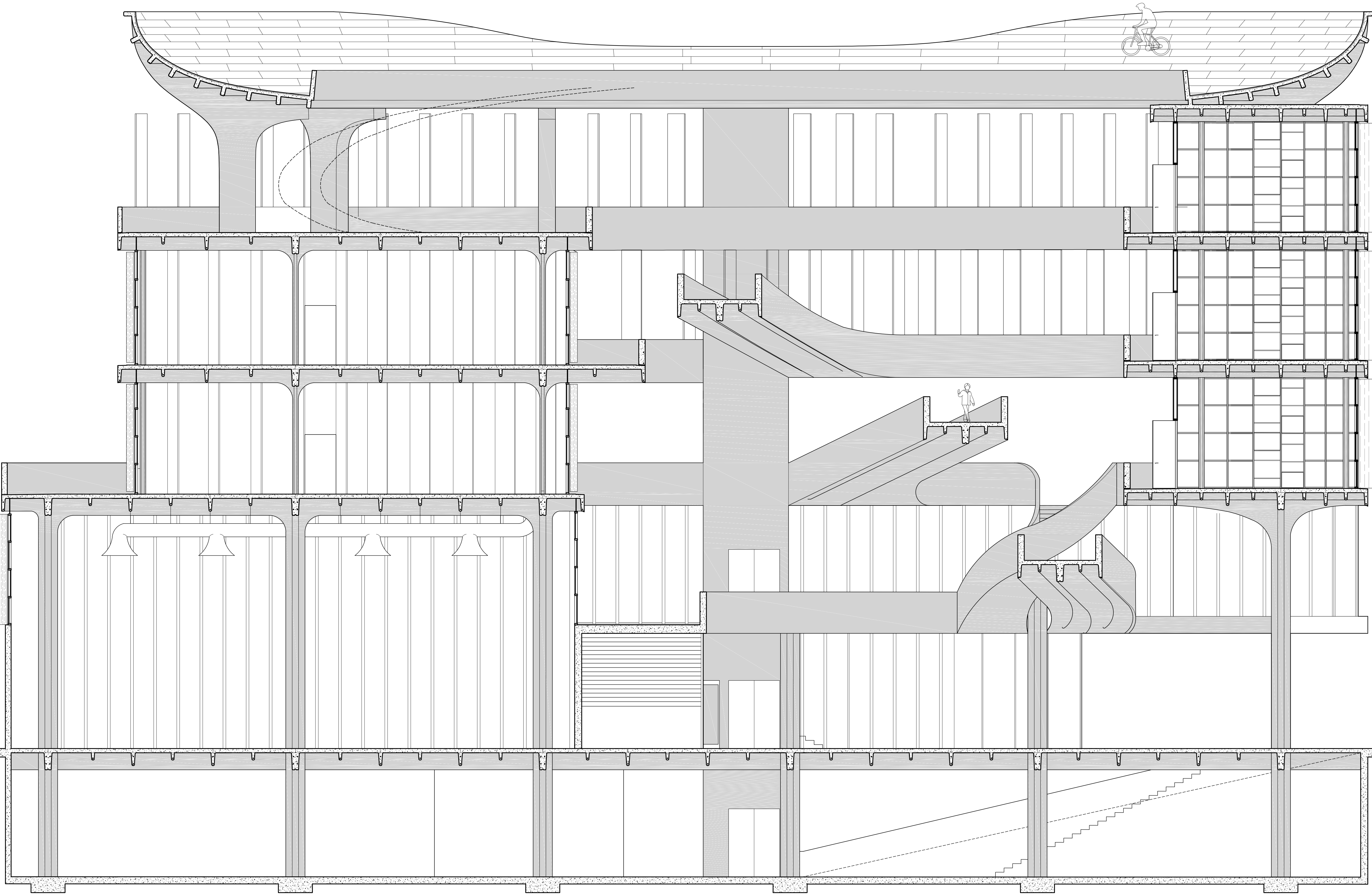
SIDE SECTION (3/16" = 1'-0")
