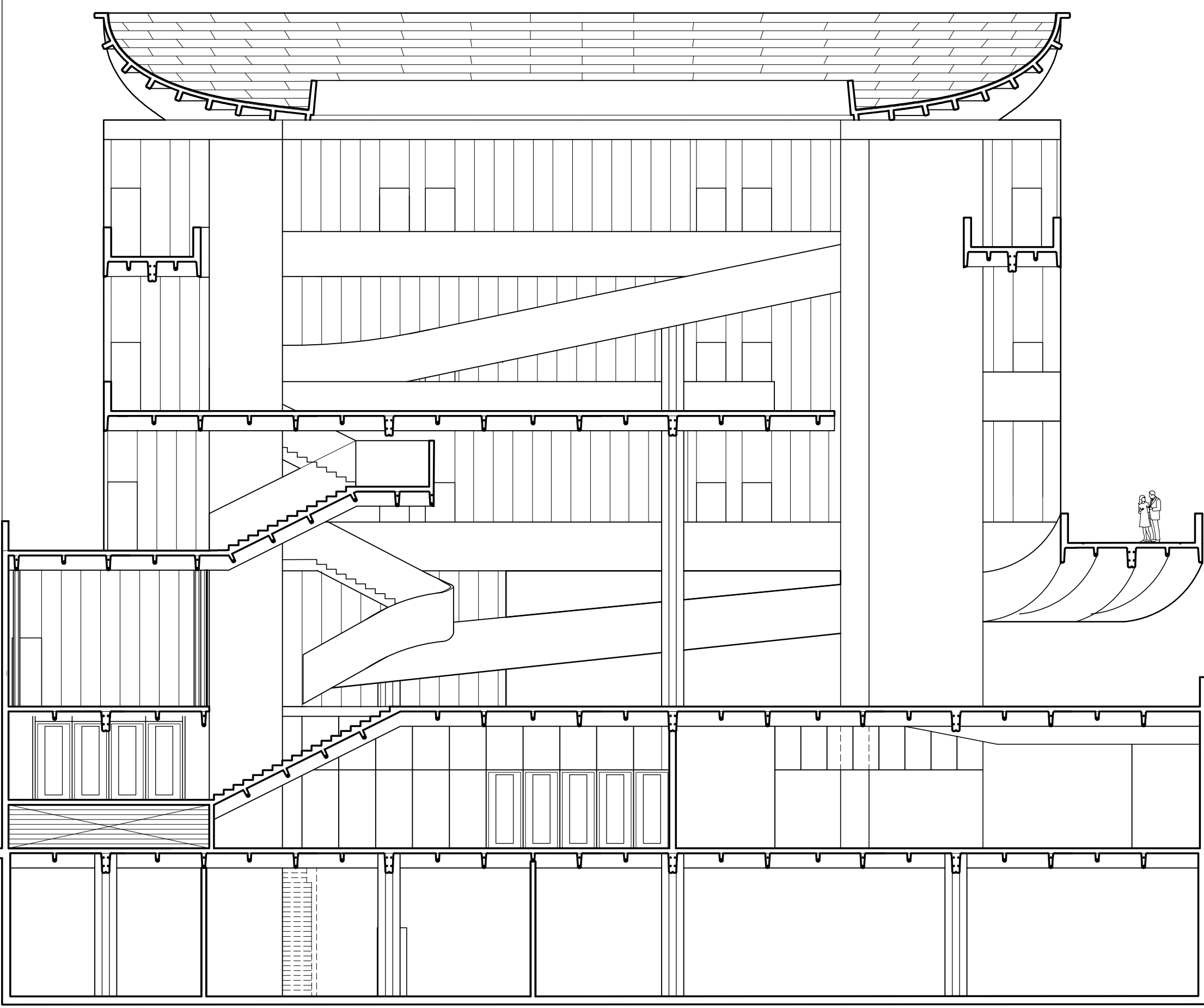
CROSS SECTION (3/32" = 1'-0")
