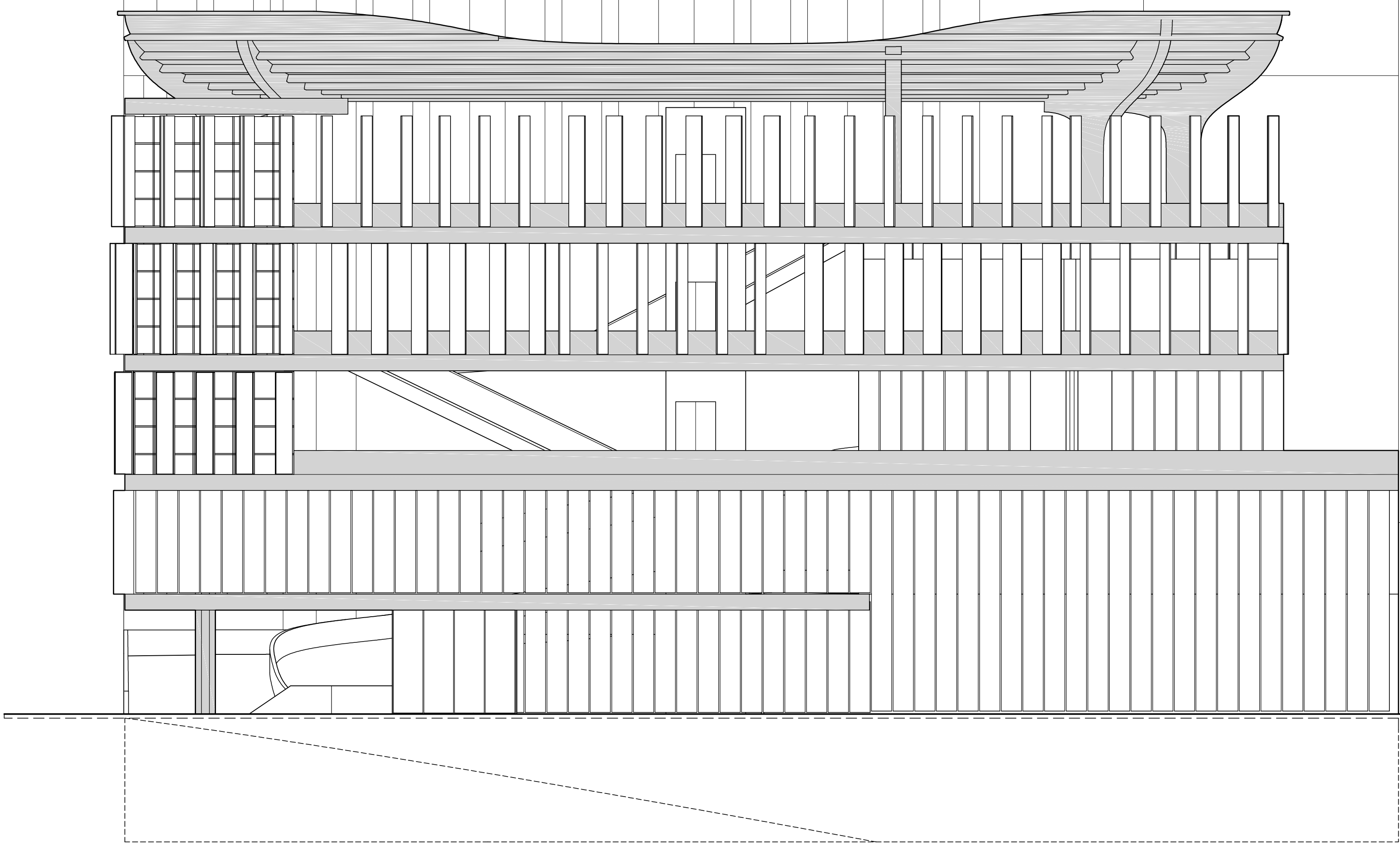
SIDE ELEVATION (3/32" = 1'-0")
